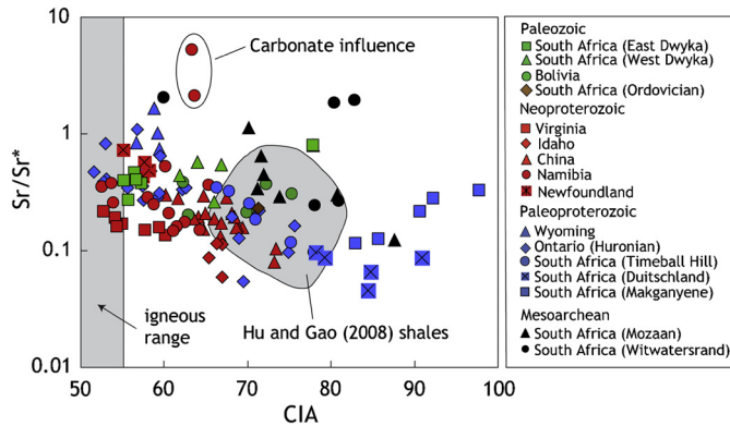
Fig. 6. Chemical index of alteration (CIA) vs. Sr depletion factor ( Sr/Sr^* = (Ce_n \cdot Nd_n)^{0.5} ) for the diamictites. CIA values between 40 and 55 are typical of fresh igneous rocks. The CIA is less than 70 for the majority of samples, but nearly all show depletion in Sr, suggesting that all samples have been influenced by chemical weathering. Sr enrichment seen in some of the Neoproterozoic Namibian samples is linked to significant carbonate content. The gray field represents post-Archean shales studied by Hu and Gao (2008), and includes some post-Archean Australian shale (PAAS, Nance and Taylor, 1976) samples, as well as samples from eastern China. (See web version of article for color figure.)
