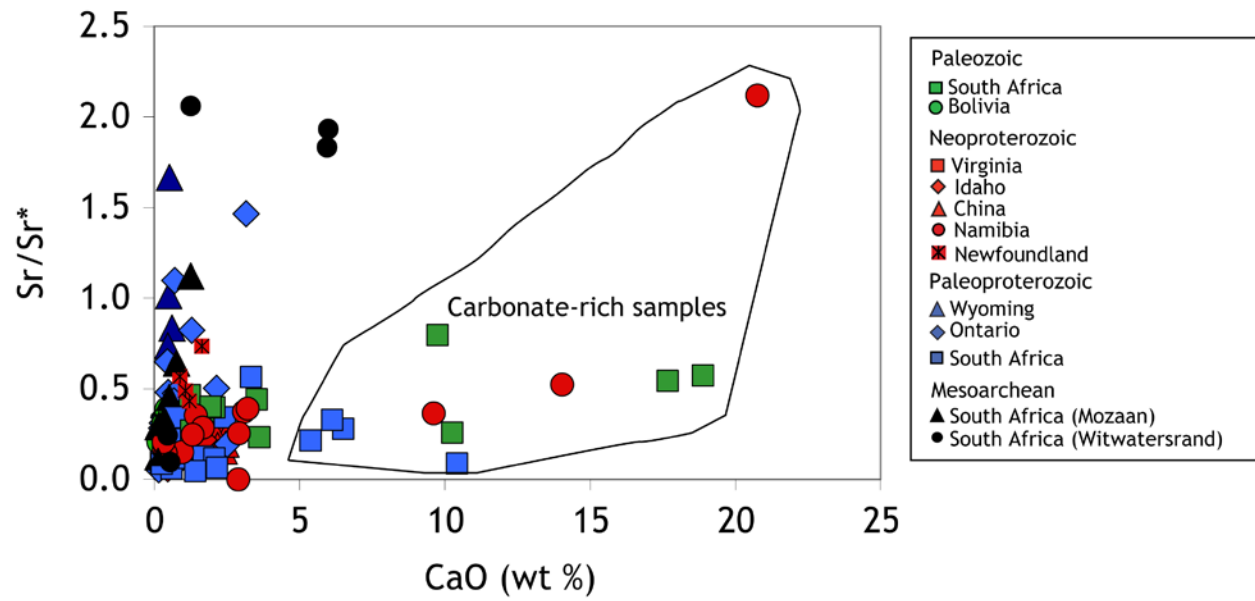
Figure A3. Sr/Sr^* vs CaO. Note that the presence of carbonate (high CaO) has limited effect on Sr enrichment. Only two carbonate-rich samples (both from Namibia, one plotting off this scale) show Sr/Sr^* > 1
