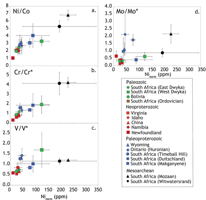
Fig. 8. Ni_{norm} vs. Ni/Co, Cr/Cr*, V/V* and Mo/Mo*. Ni_{norm} is Ni concentration normalized to Rudnick and Gao (2003) average UCC Al_2O_3 of 15.26% ( Ni_{norm} = 15.26/Al_2O_{3measured} * Ni_{measured} ). Good correlation between Ni_{norm} and Ni/Co and Cr/Cr* is interpreted as an intracrustal differentiation trend due to the similar igneous partition coefficients between Ni and Cr. However, Ni_{norm} is decoupled from V/V* and Mo/Mo* due to the influence of oxidative weathering on V and Mo behavior. (See web version of article for color figure.)
