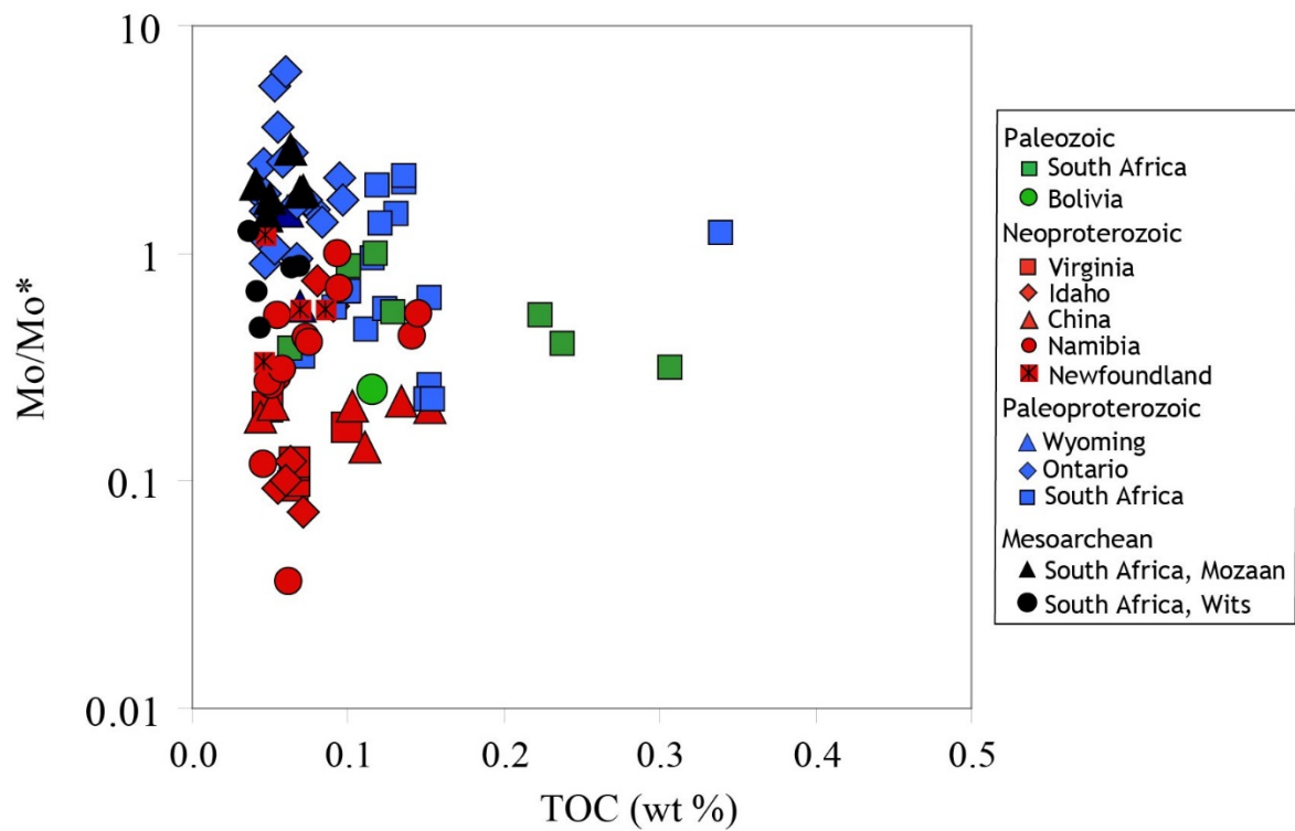
Figure A6 – Mo/Mo* (Mo enrichment or depletion relative to LREE) vs. total organic carbon (TOC). The lack of correlation suggests that differences in Mo are due to the dissolution or survival of Mo-bearing detrital minerals, depending on the oxygen levels, rather than authigenic enrichment or lack thereof.
